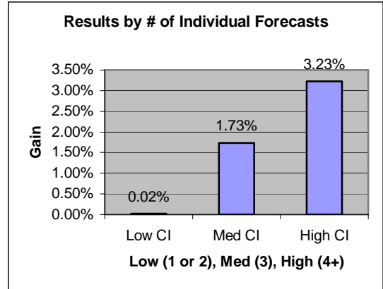
Figure 7. Results by Number of Individual Forecasts
